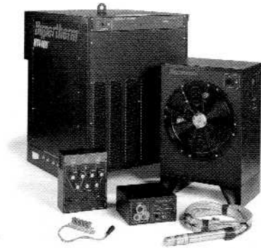
HySpeedHT4400 with accessories
